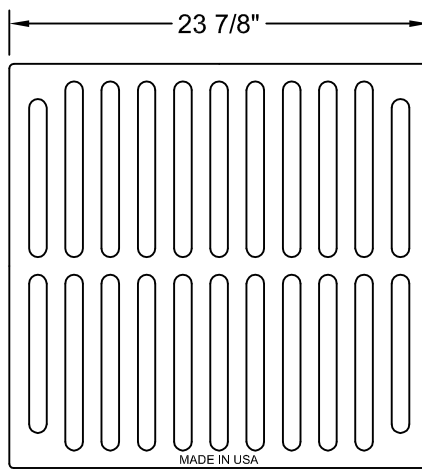
PLAN VIEW #1604 C.I. GRATE
