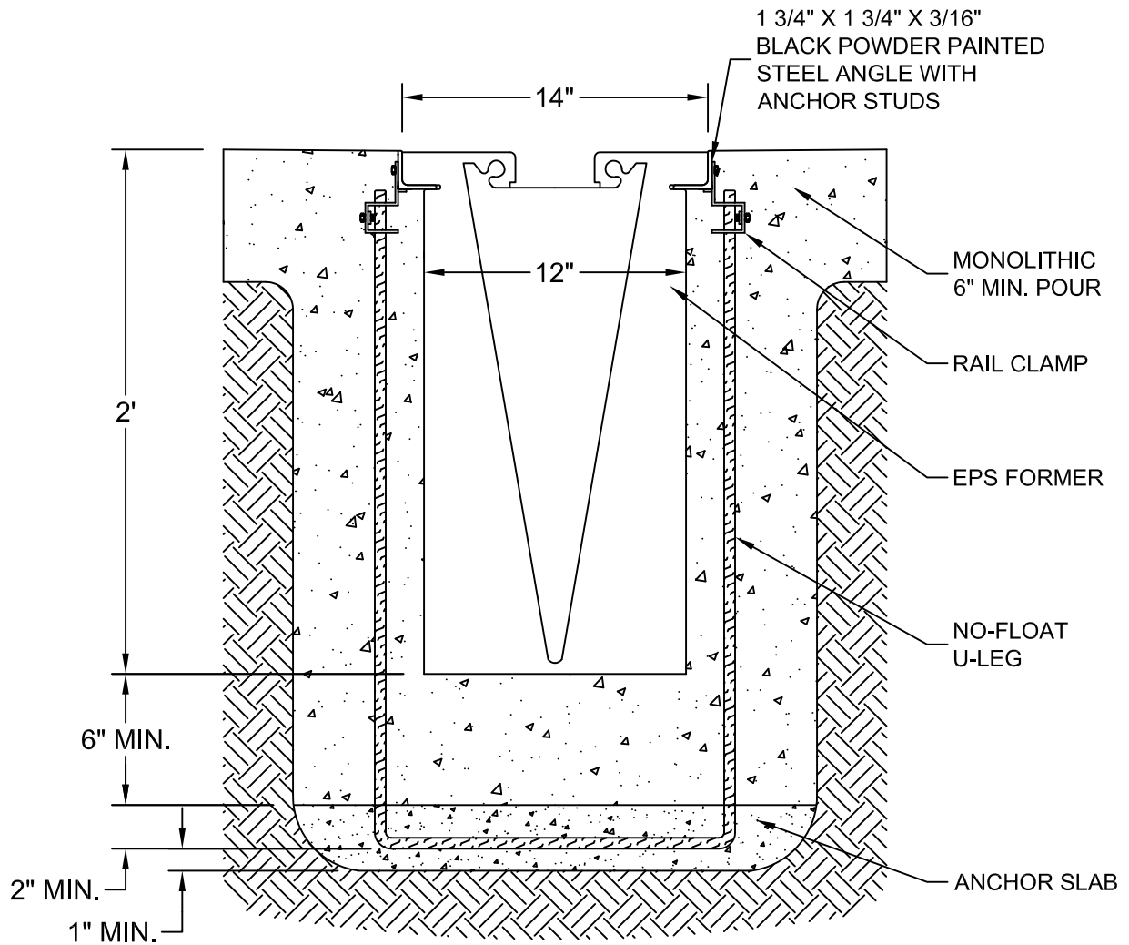
END CROSS SECTION VIEW
