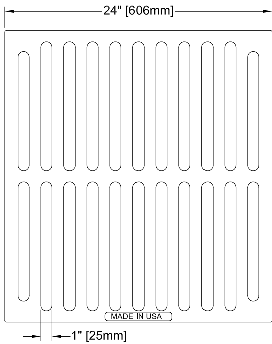
GRATE TOP VIEW (ROTATED 90°)
