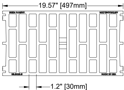
GRATE TOP VIEW (ROTATED 90°)
