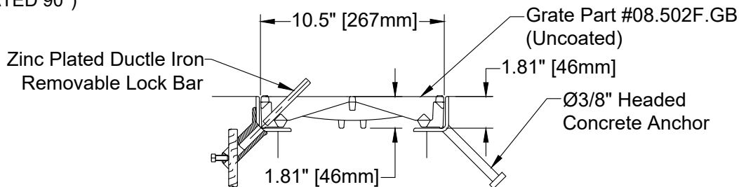
GRATE END VIEW
