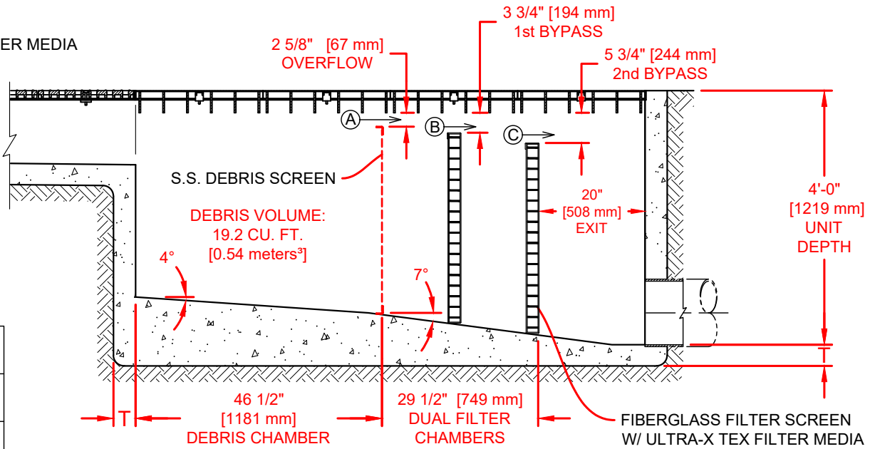
CROSS SECTIONAL VIEW
