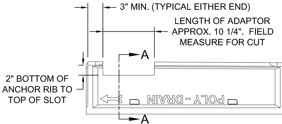
CHANNEL MODIFICATIONS FOR Ø8" PVC ADAPTOR
