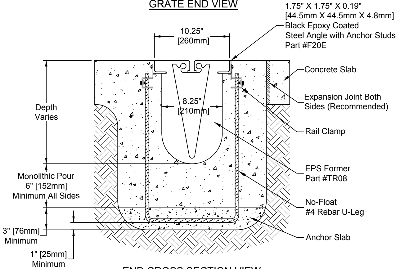
END CROSS SECTION VIEW
