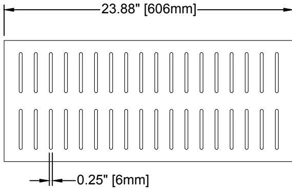
GRATE TOP VIEW (ROTATED 90°)
