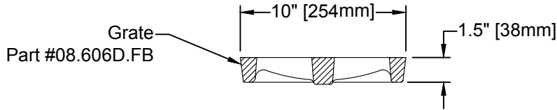
GRATE END VIEW
